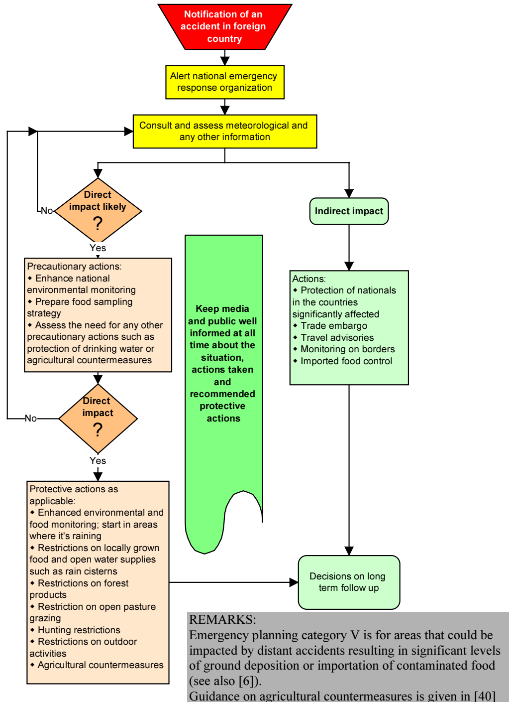
FIG. V1. Response scheme for country in emergency planning category v in case of severe nuclear accident.
