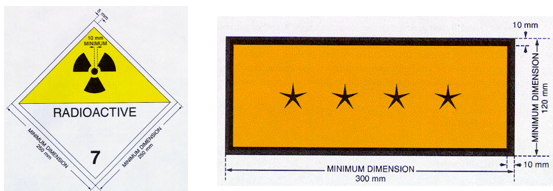
FIG IV2. Placarding signs
