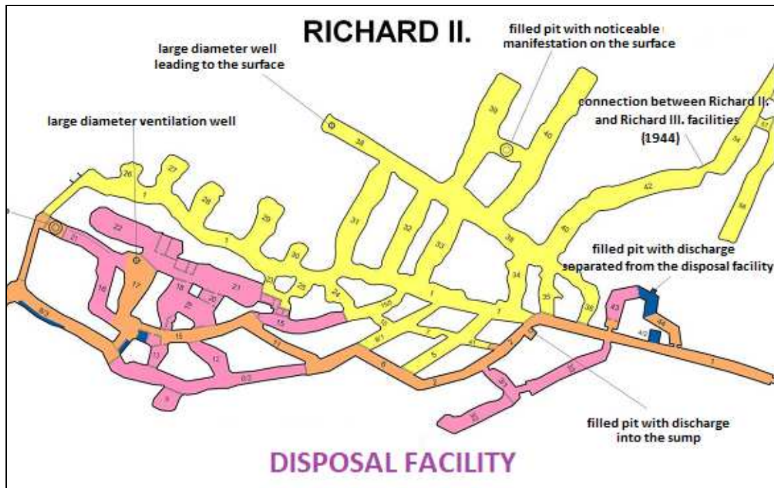
Fig. 4.6 RAW disposal facility Richard – layout (disposal chambers marked in violet)
