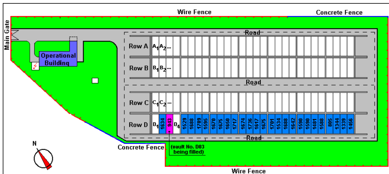
Fig. 4.8 Ground plan and current filling of the disposal units in RAW disposal facility Dukovany with casks (200 l drums, MOZAIK casks and box pallets; it does not include solid, unconditioned RAW) as at December 31, 2019
